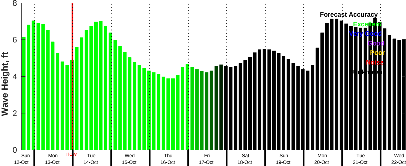
CMEMS Wave Forecast for NDBC 46215 from 12-Oct-2025 16:00:00 to 22-Oct-2025 16:00:00
