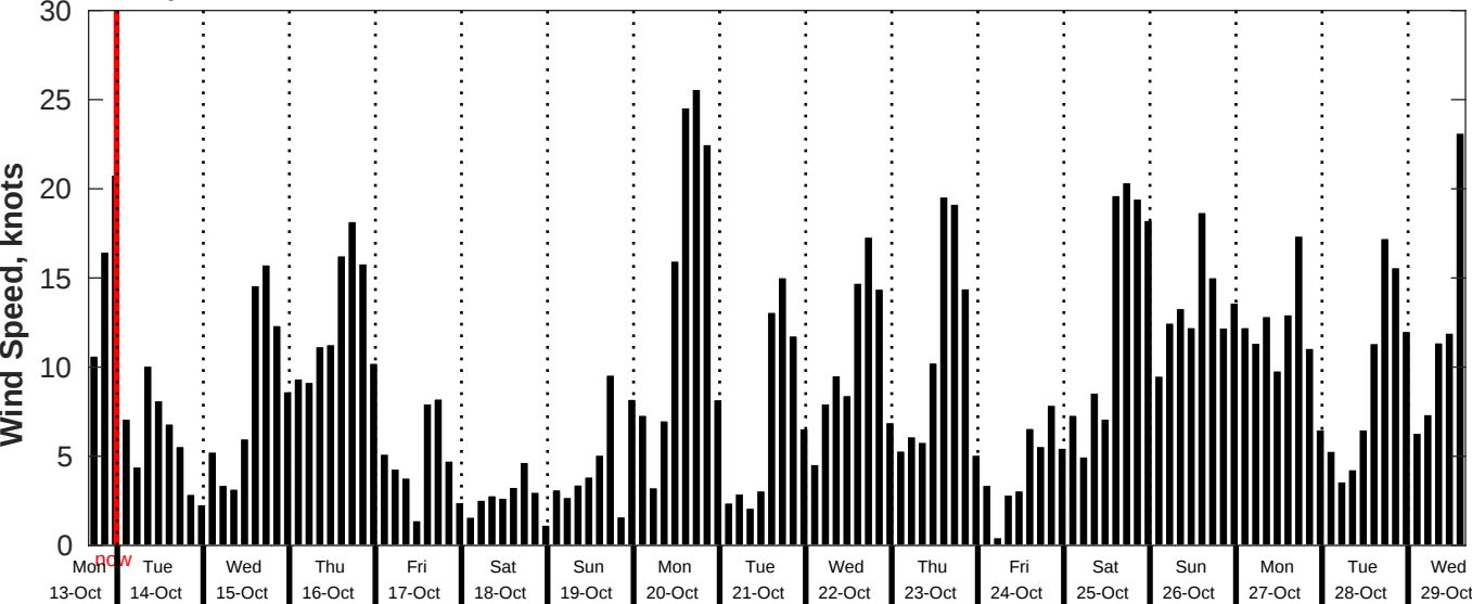
GFS Wind Speed Forecast for NDBC 46215 from 13-Oct-2025 16:00:00 to 29-Oct-2025 16:00:00
