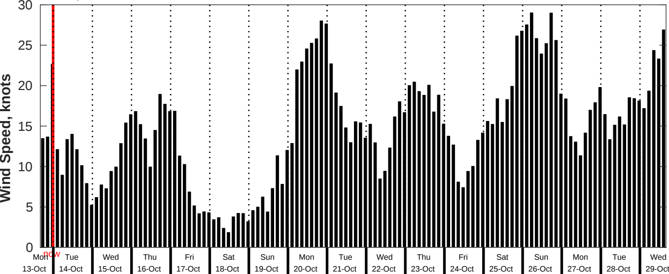
GFS Wind Speed Forecast for NDBC 46259 from 13-Oct-2025 16:00:00 to 29-Oct-2025 16:00:00
