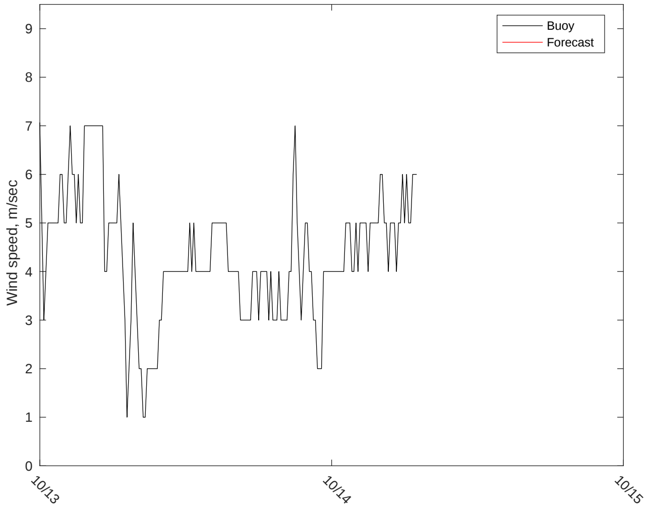
NDBC 51000 vs GFS Winds: 10 to 16 day forecast
