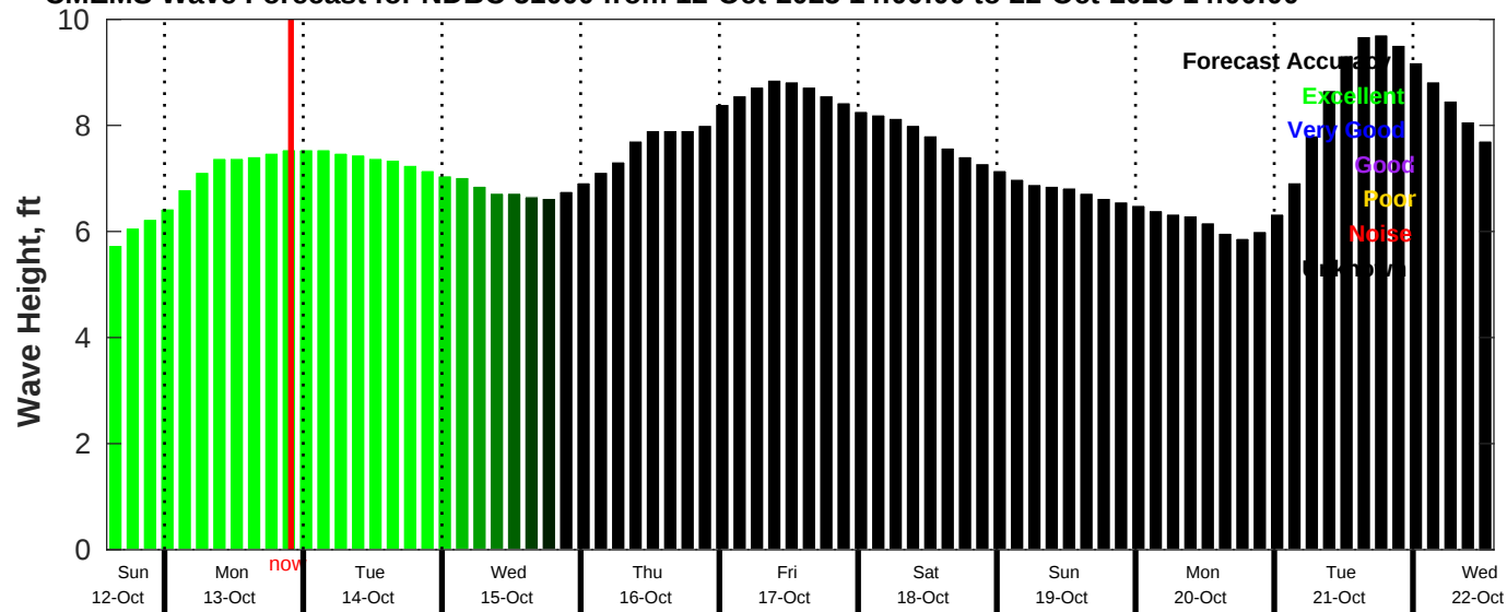
CMEMS Wave Forecast for NDBC 51000 from 12-Oct-2025 14:00:00 to 22-Oct-2025 14:00:00
