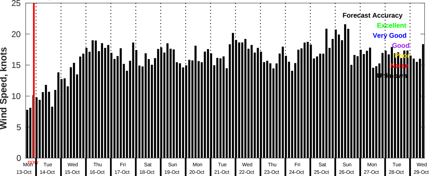
GFS Wind Speed Forecast for NDBC 51000 from 13-Oct-2025 14:00:00 to 29-Oct-2025 14:00:00
