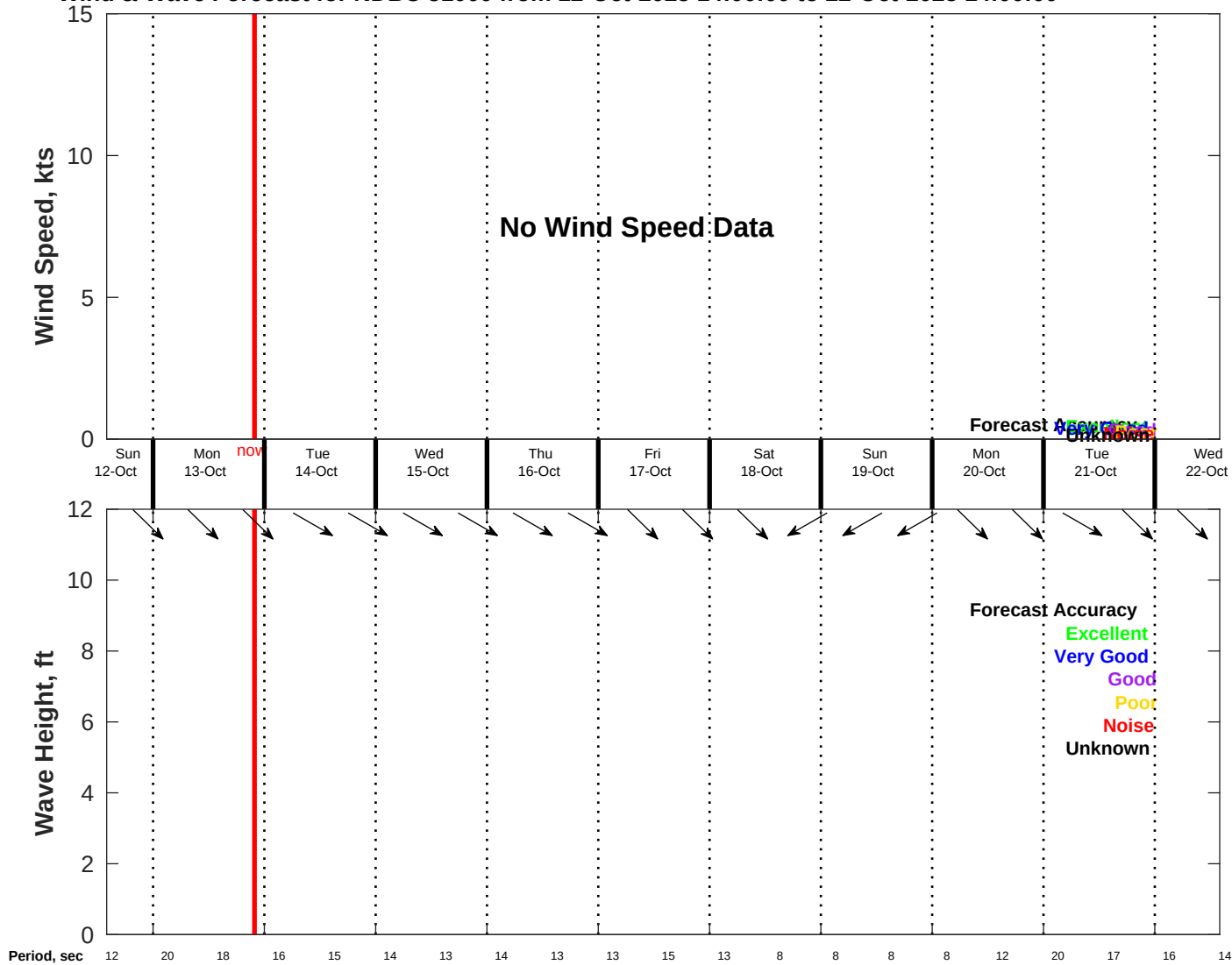
Wind & Wave Forecast for NDBC 51000 from 12-Oct-2025 14:00:00 to 22-Oct-2025 14:00:00
