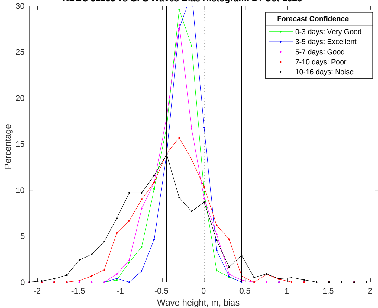
NDBC 51209 vs GFS Waves Bias Histogram: 14-Oct-2025
