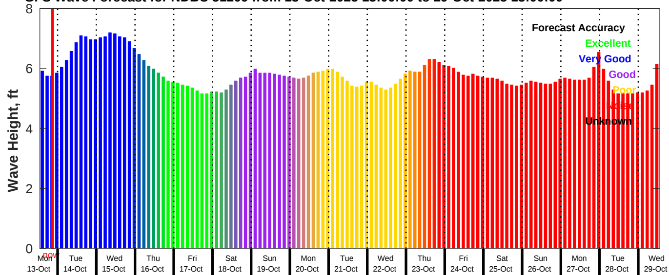
GFS Wave Forecast for NDBC 51209 from 13-Oct-2025 13:00:00 to 29-Oct-2025 13:00:00
