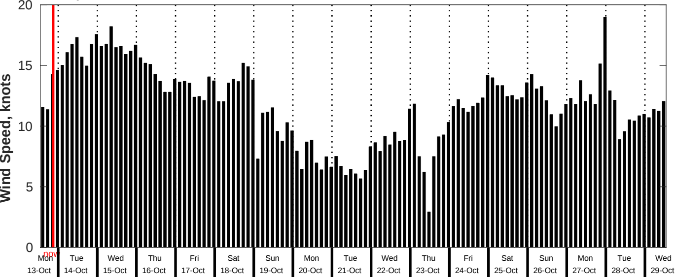
GFS Wind Speed Forecast for NDBC 51209 from 13-Oct-2025 13:00:00 to 29-Oct-2025 13:00:00
