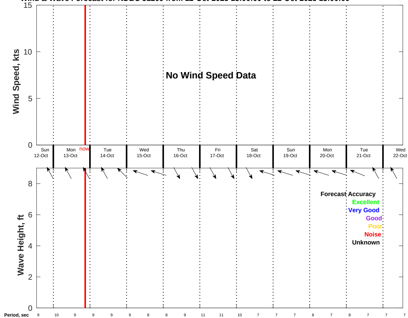
Wind & Wave Forecast for NDBC 51209 from 12-Oct-2025 13:00:00 to 22-Oct-2025 13:00:00
