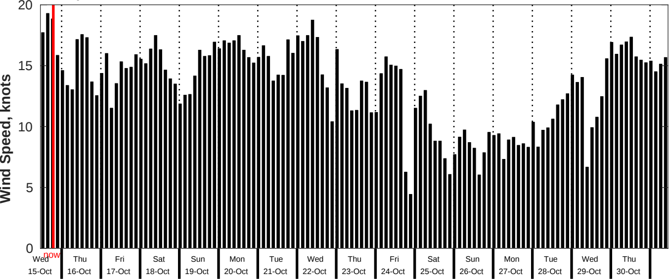
GFS Wind Speed Forecast for NDBC 52211 from 14-Oct-2025 11:00:00 to 30-Oct-2025 11:00:00
