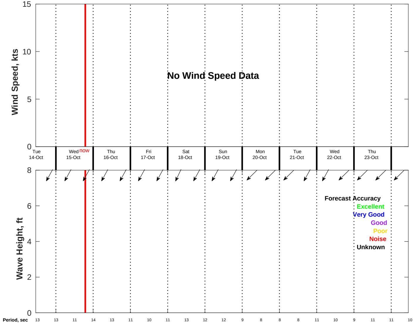
Wind & Wave Forecast for NDBC 52211 from 13-Oct-2025 11:00:00 to 23-Oct-2025 11:00:00
