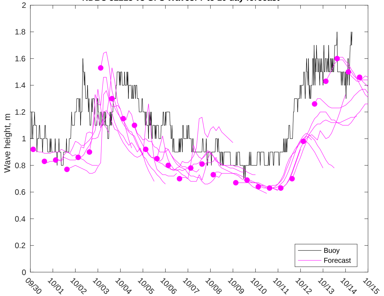
NDBC 52213 vs GFS Waves: 7 to 10 day forecast
