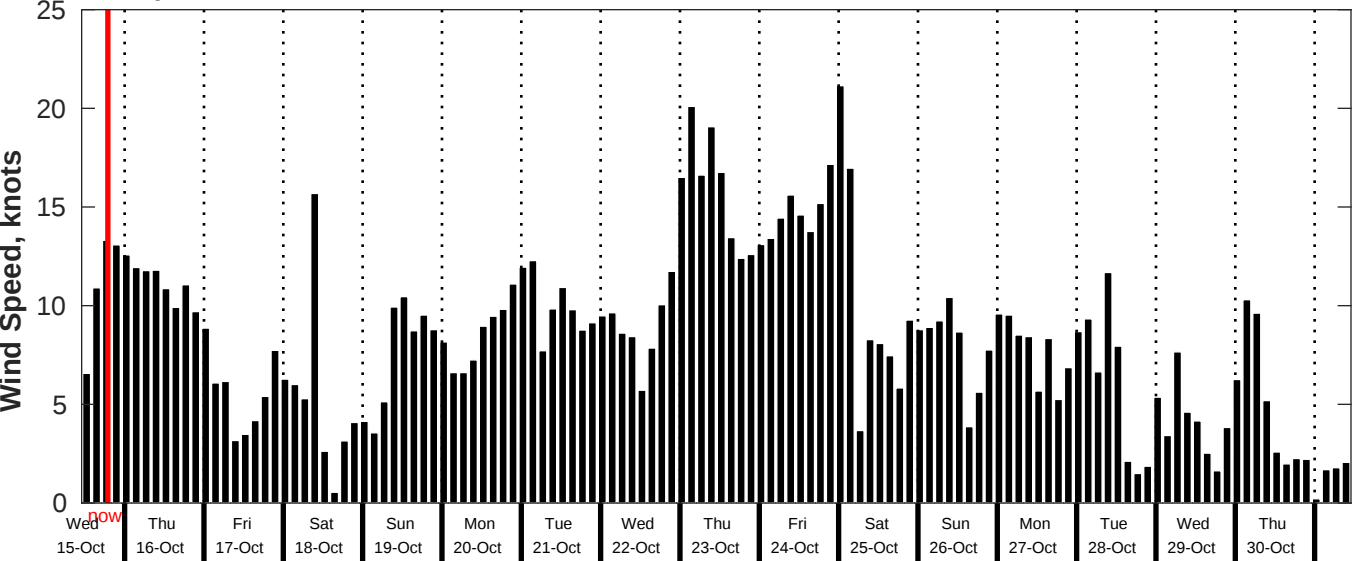
GFS Wind Speed Forecast for NDBC 52213 from 14-Oct-2025 11:00:00 to 30-Oct-2025 11:00:00
