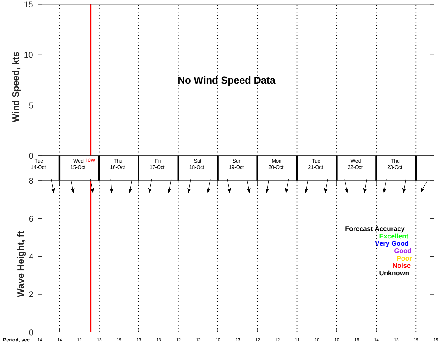
Wind & Wave Forecast for NDBC 52213 from 13-Oct-2025 11:00:00 to 23-Oct-2025 11:00:00
