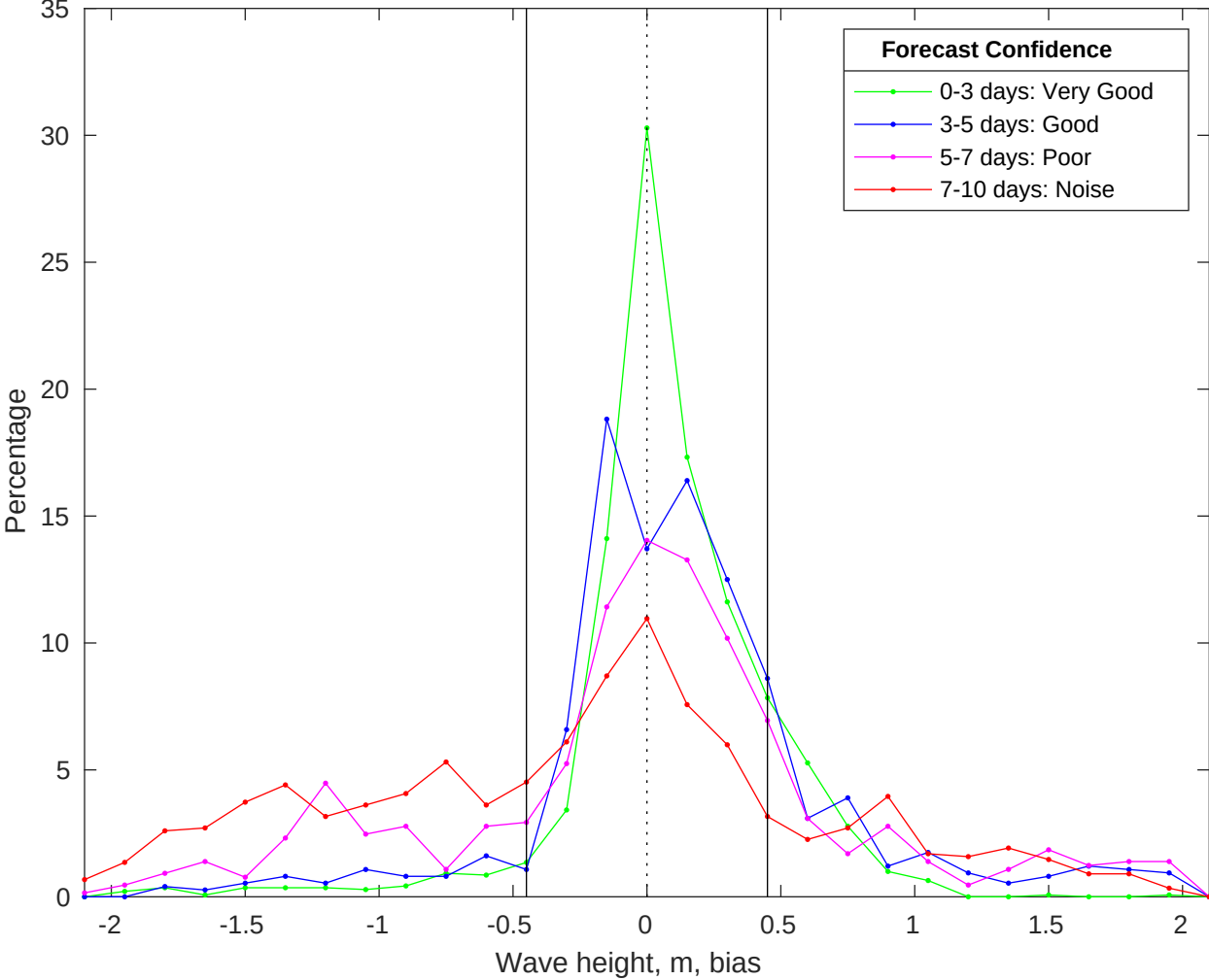
NDBC 41013 vs CMEMS Waves Bias Histogram: 13-Oct-2025
