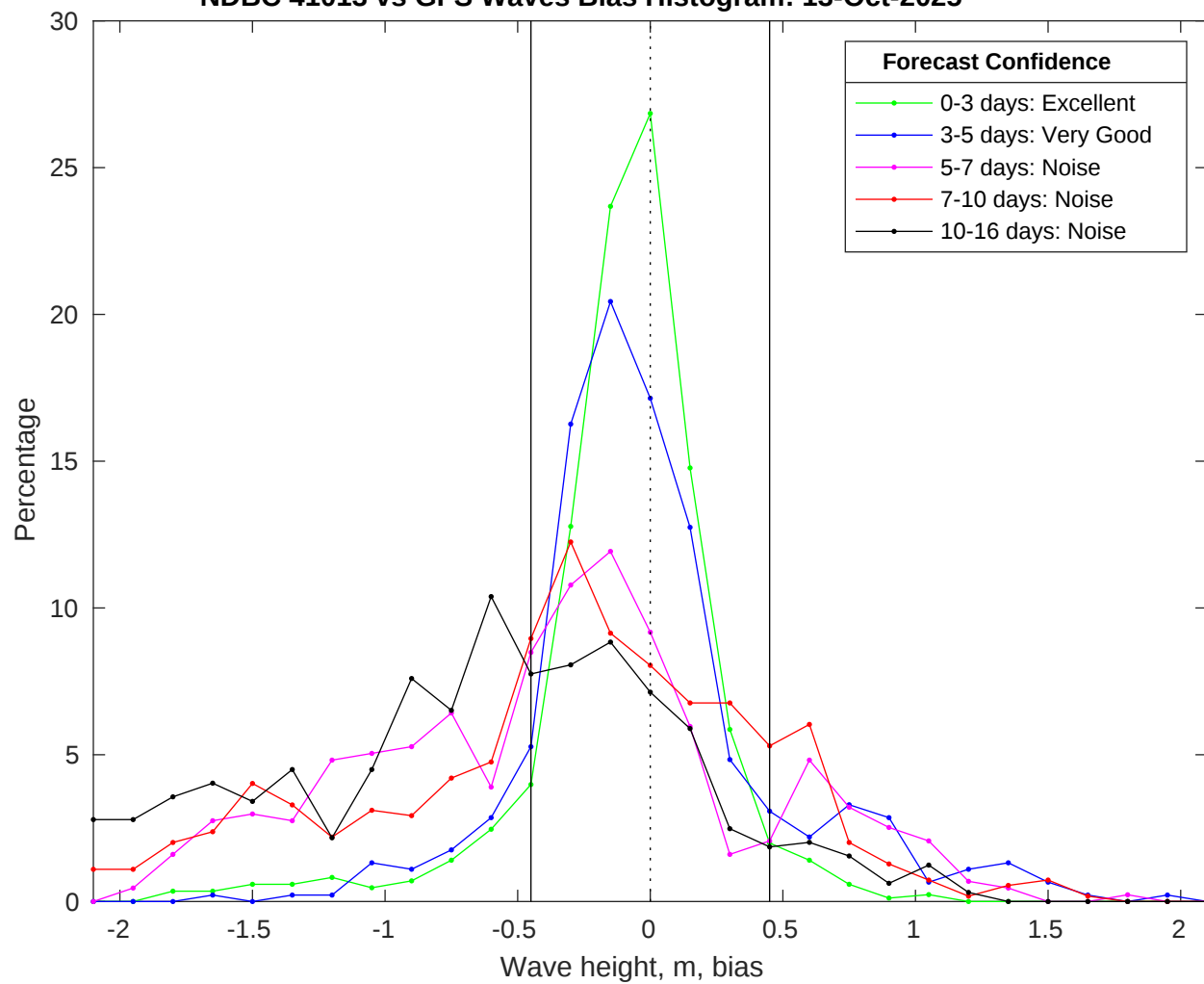
NDBC 41013 vs GFS Waves Bias Histogram: 13-Oct-2025
