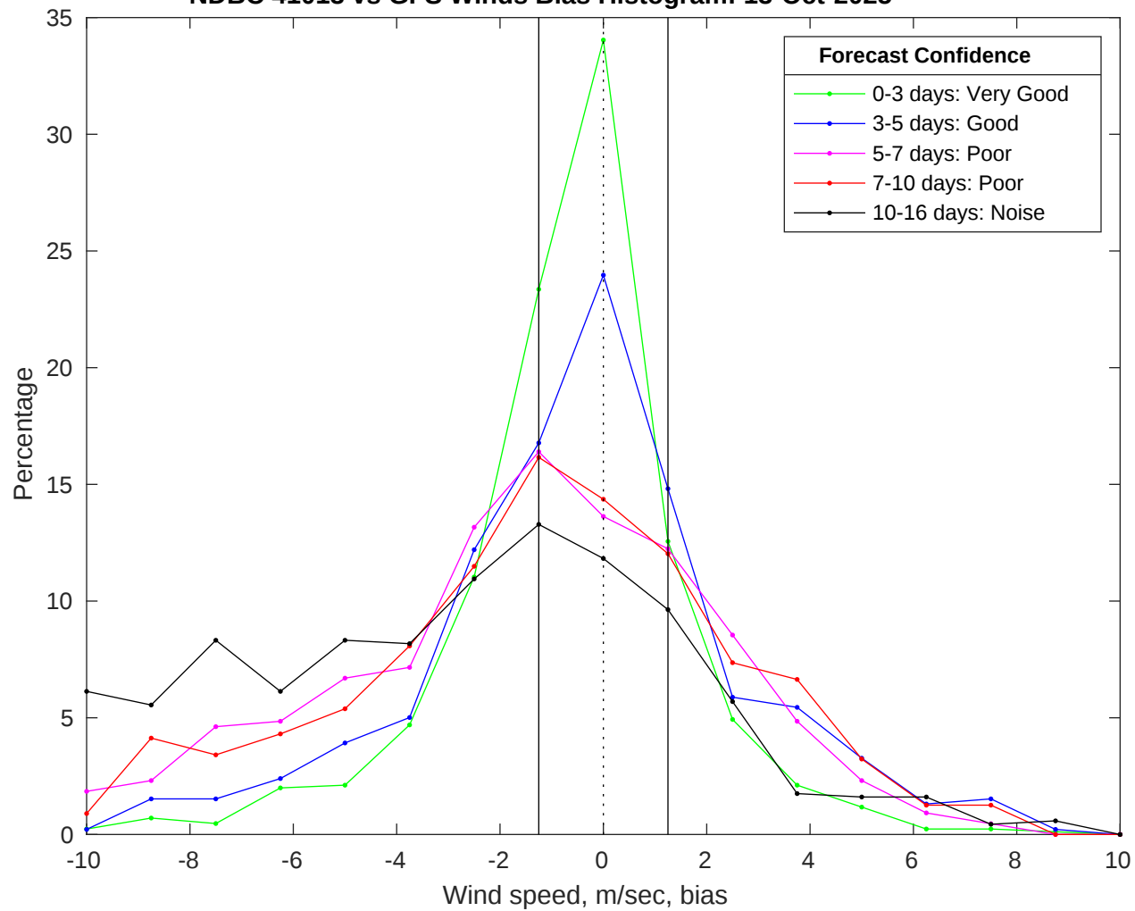
NDBC 41013 vs GFS Winds Bias Histogram: 13-Oct-2025
