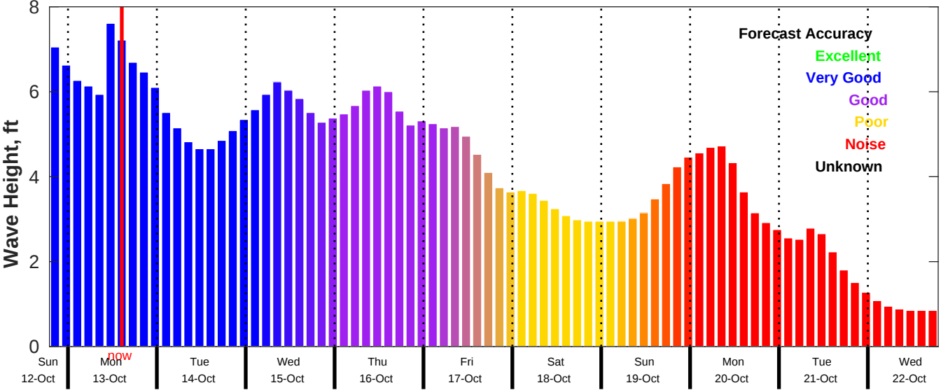
CMEMS Wave Forecast for NDBC 41013 from 12-Oct-2025 19:00:00 to 22-Oct-2025 19:00:00
