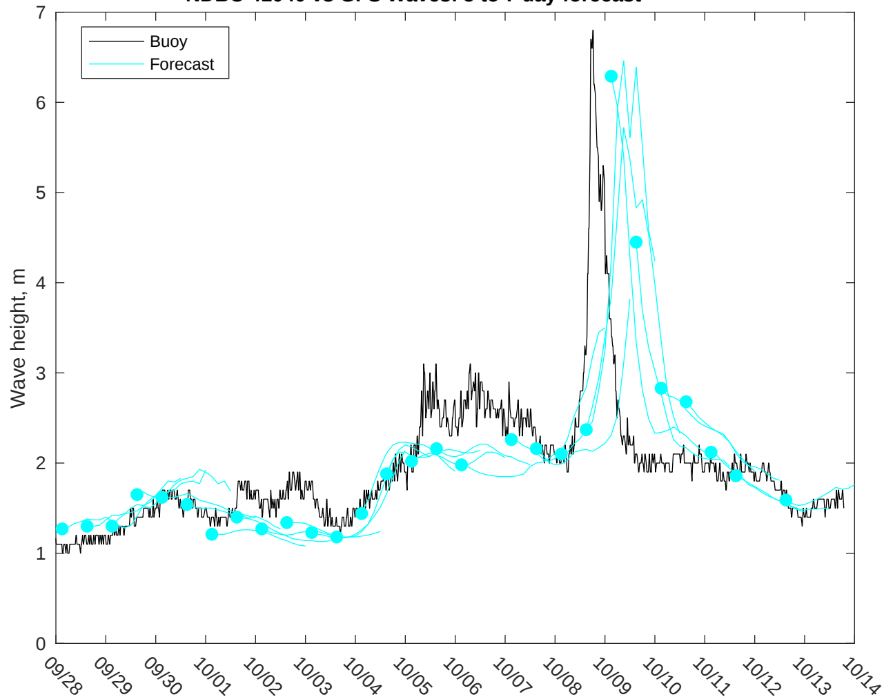
NDBC 41040 vs GFS Waves: 5 to 7 day forecast
