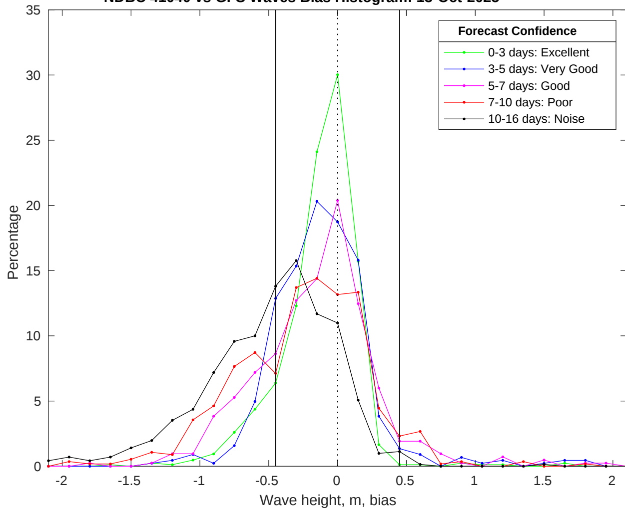
NDBC 41040 vs GFS Waves Bias Histogram: 13-Oct-2025
