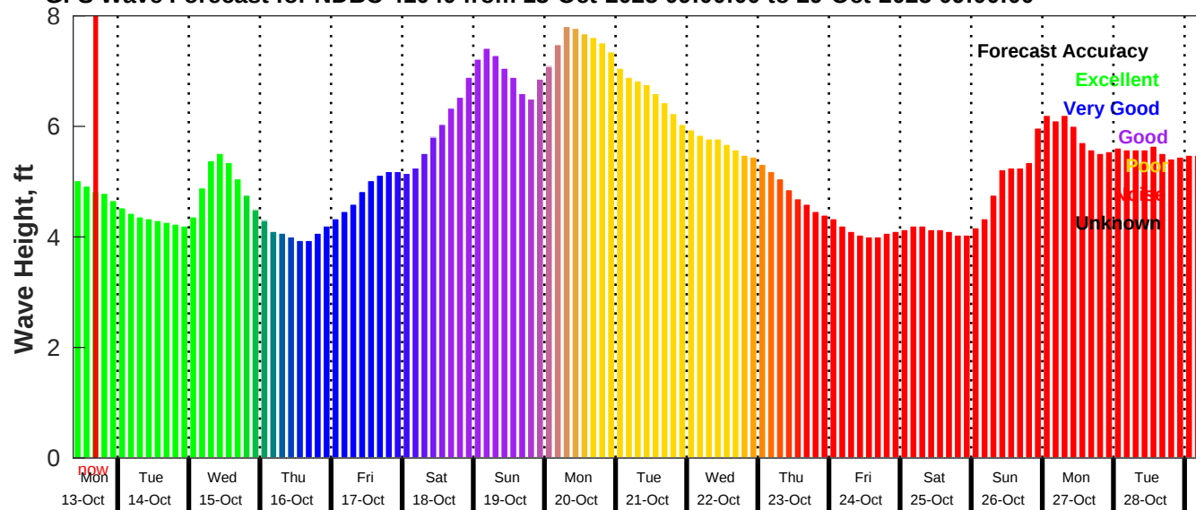
GFS Wave Forecast for NDBC 41040 from 13-Oct-2025 09:00:00 to 29-Oct-2025 09:00:00
