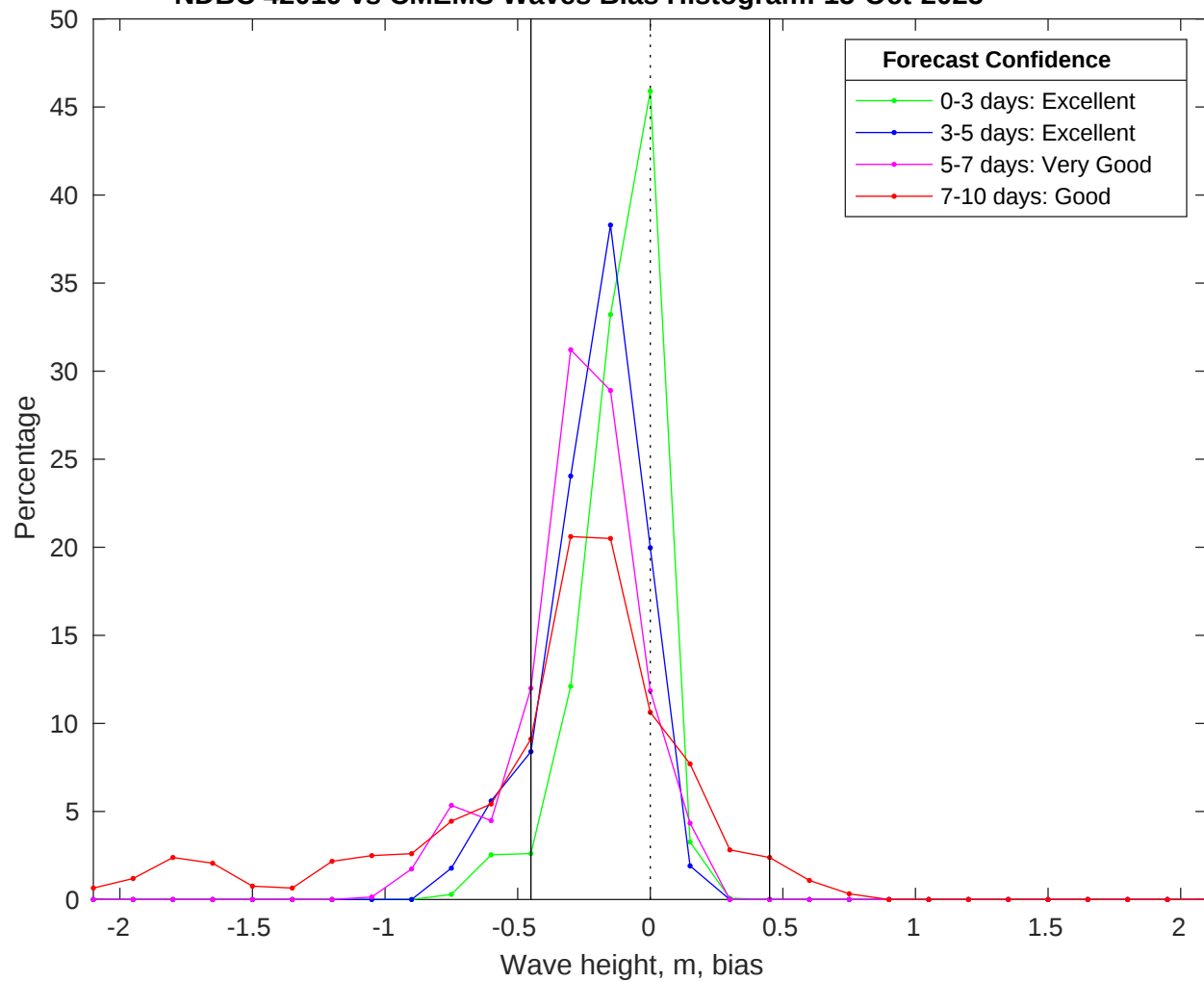
NDBC 42019 vs CMEMS Waves Bias Histogram: 15-Oct-2025
