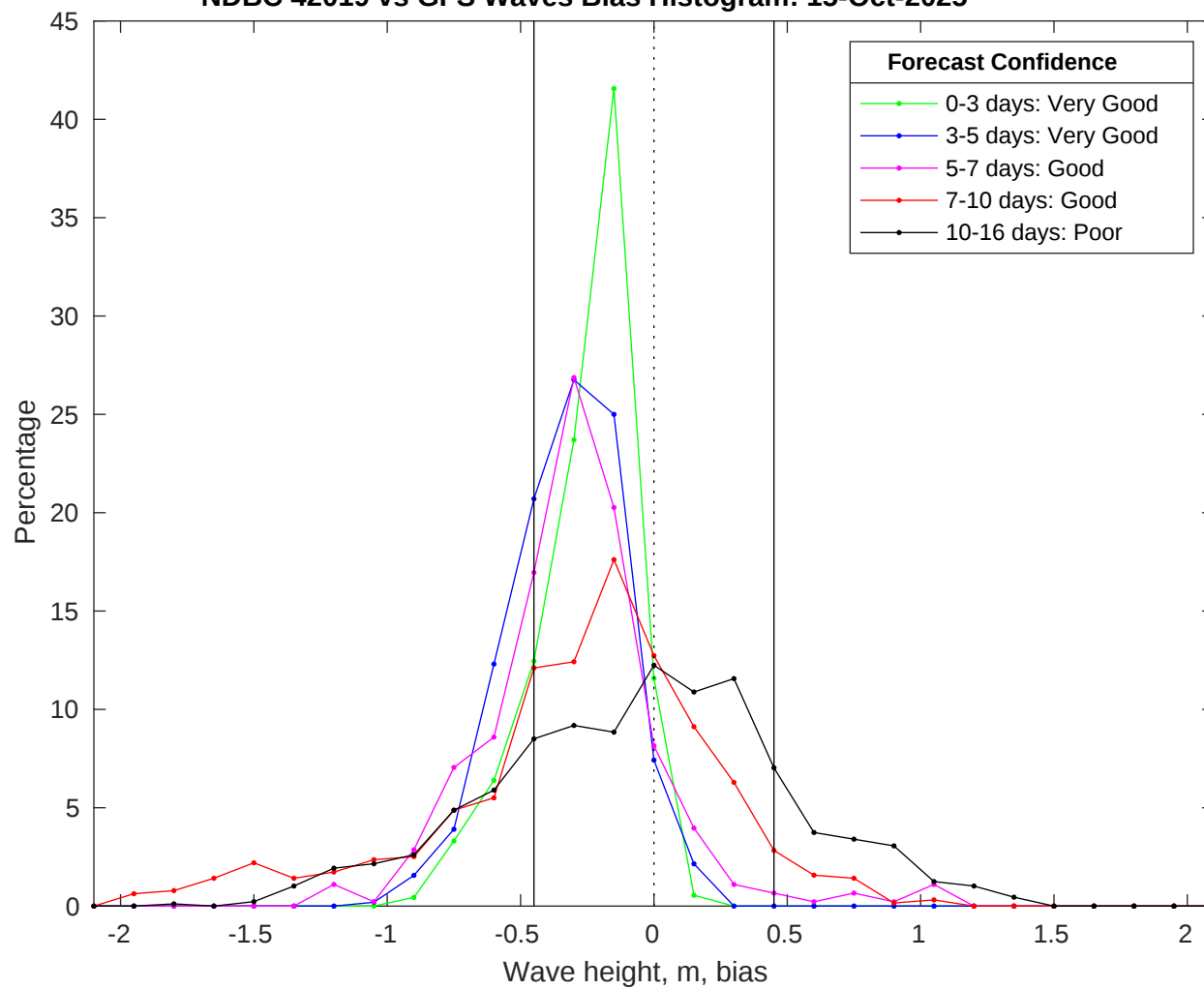
NDBC 42019 vs GFS Waves Bias Histogram: 15-Oct-2025
