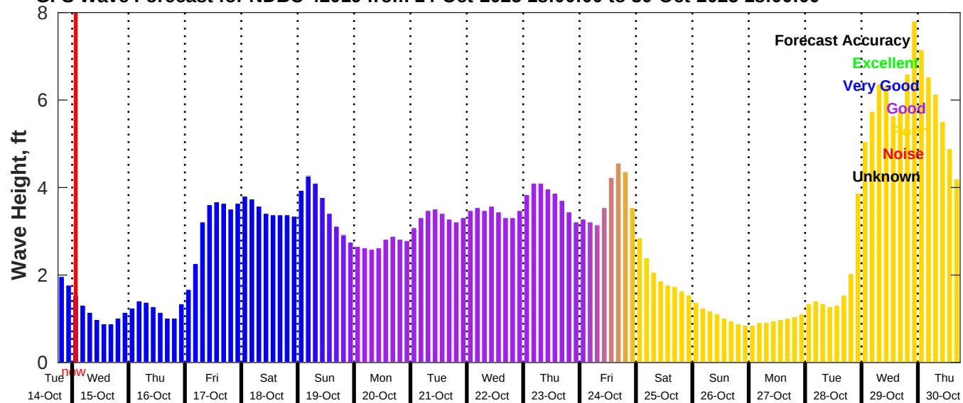
GFS Wave Forecast for NDBC 42019 from 14-Oct-2025 18:00:00 to 30-Oct-2025 18:00:00
