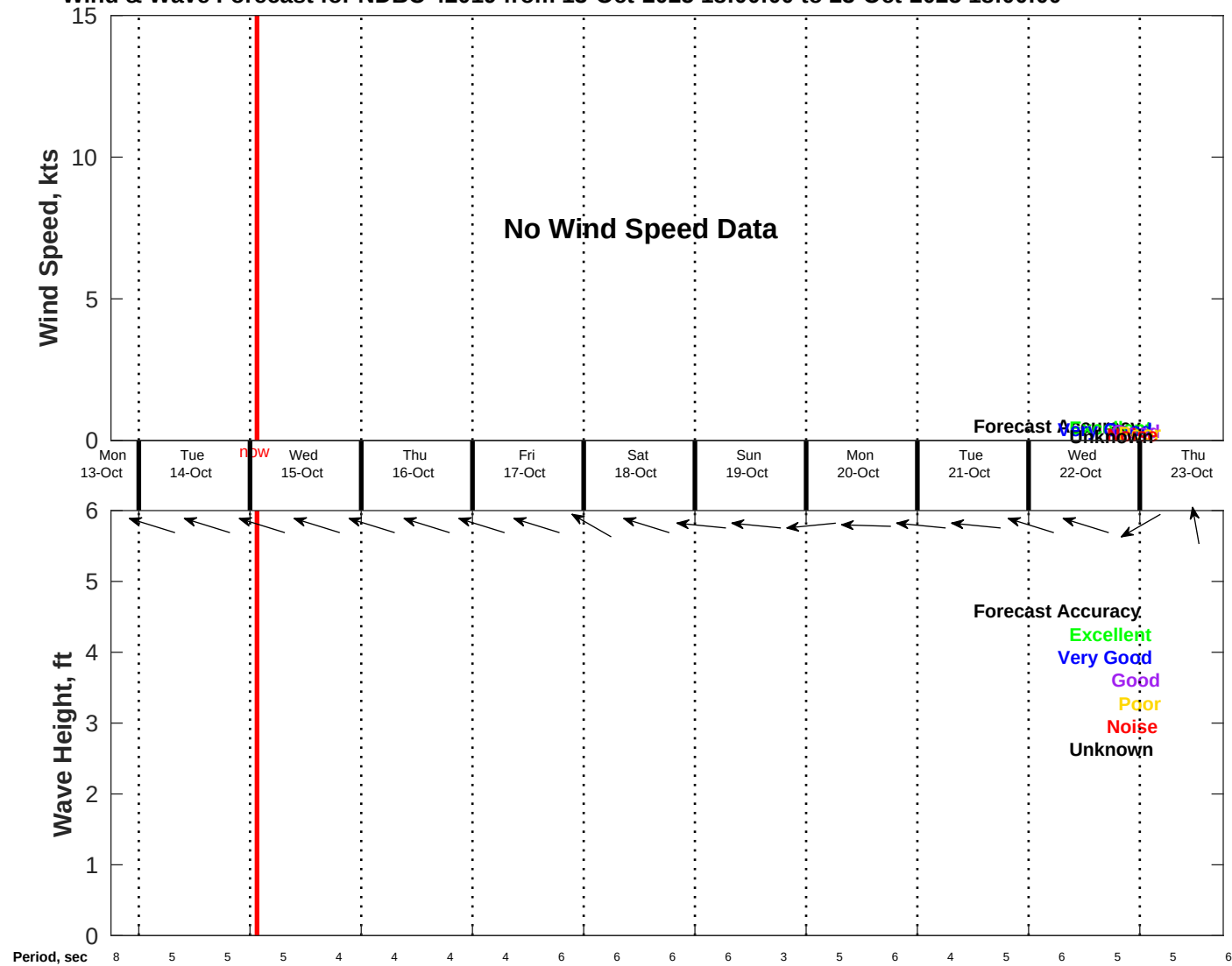
Wind & Wave Forecast for NDBC 42019 from 13-Oct-2025 18:00:00 to 23-Oct-2025 18:00:00
