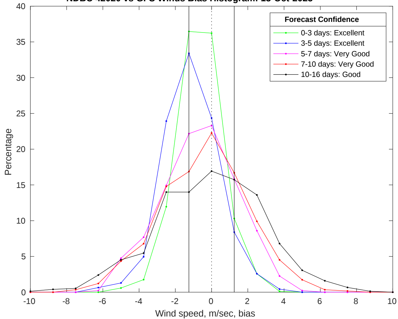
NDBC 42020 vs GFS Winds Bias Histogram: 13-Oct-2025
