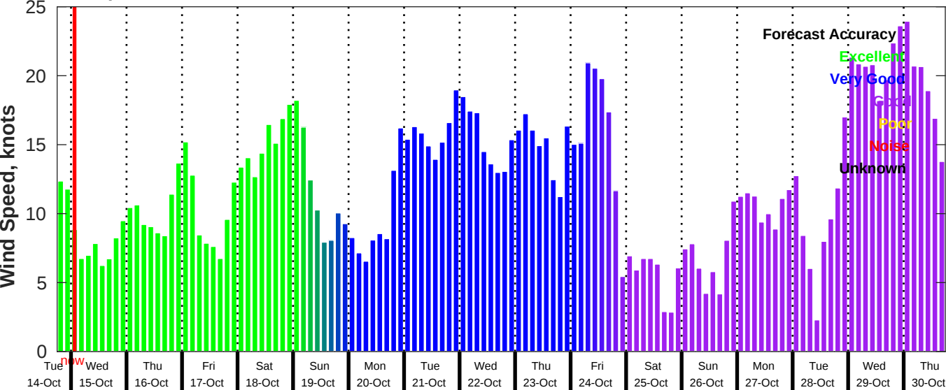
GFS Wind Speed Forecast for NDBC 42020 from 14-Oct-2025 18:00:00 to 30-Oct-2025 18:00:00
