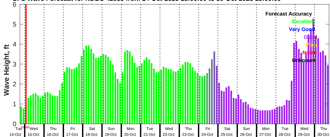
GFS Wave Forecast for NDBC 42035 from 14-Oct-2025 18:00:00 to 30-Oct-2025 18:00:00
