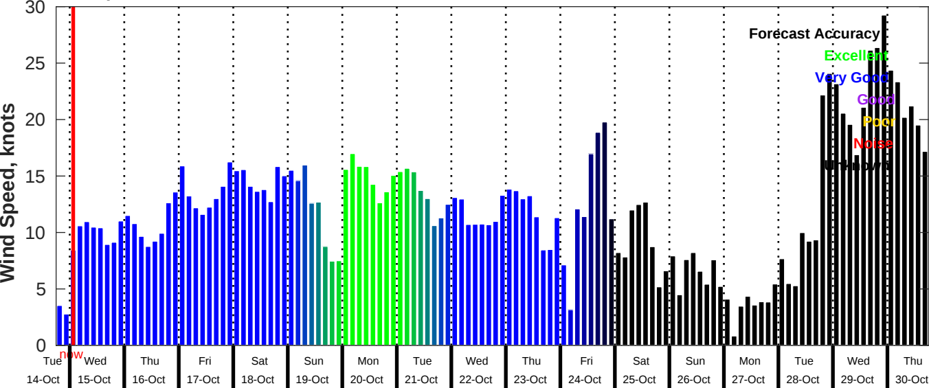
GFS Wind Speed Forecast for NDBC 42035 from 14-Oct-2025 18:00:00 to 30-Oct-2025 18:00:00
