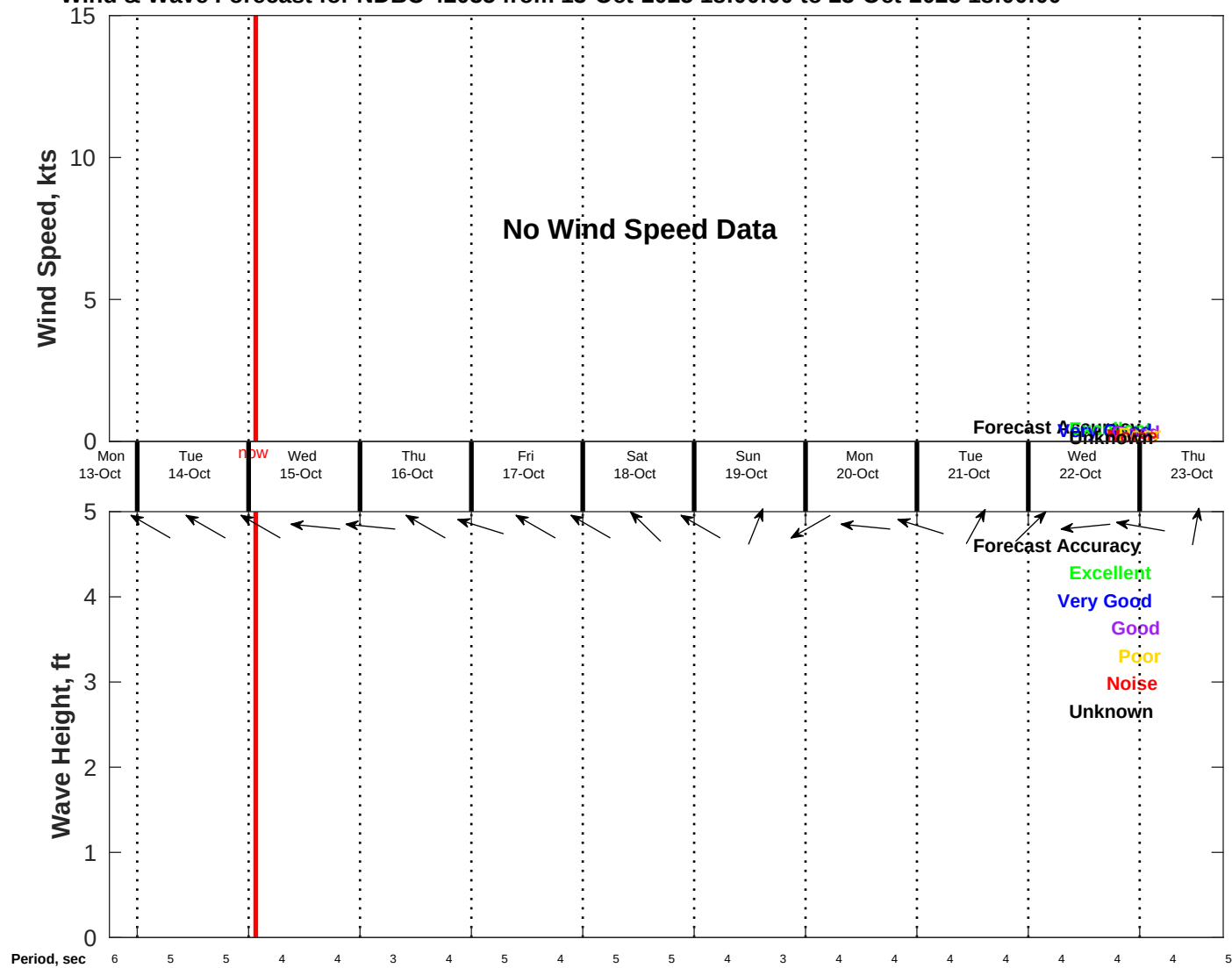
Wind & Wave Forecast for NDBC 42035 from 13-Oct-2025 18:00:00 to 23-Oct-2025 18:00:00
