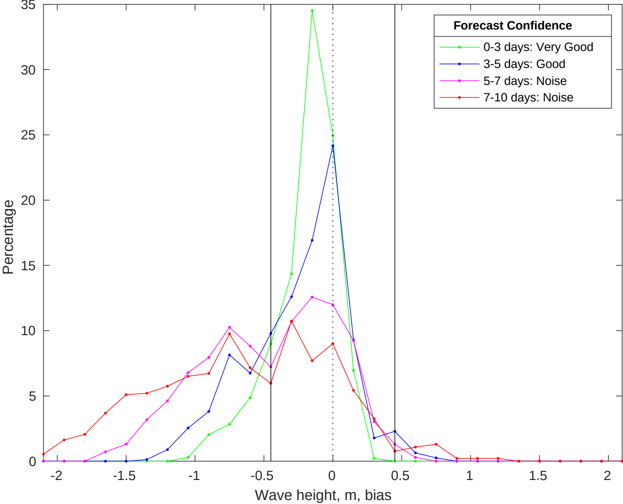
NDBC 42036 vs CMEMS Waves Bias Histogram: 15-Oct-2025
