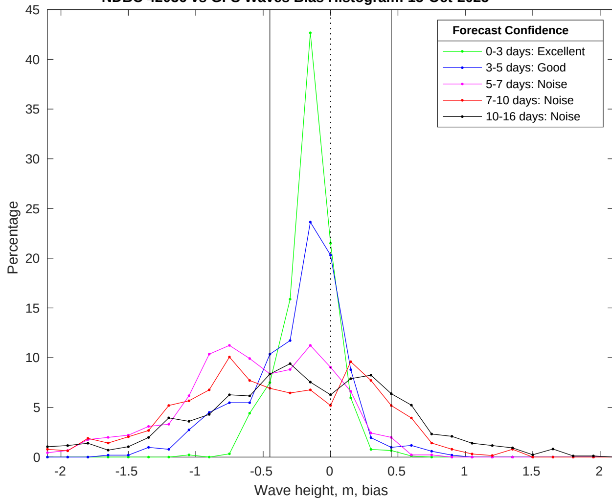
NDBC 42036 vs GFS Waves Bias Histogram: 15-Oct-2025
