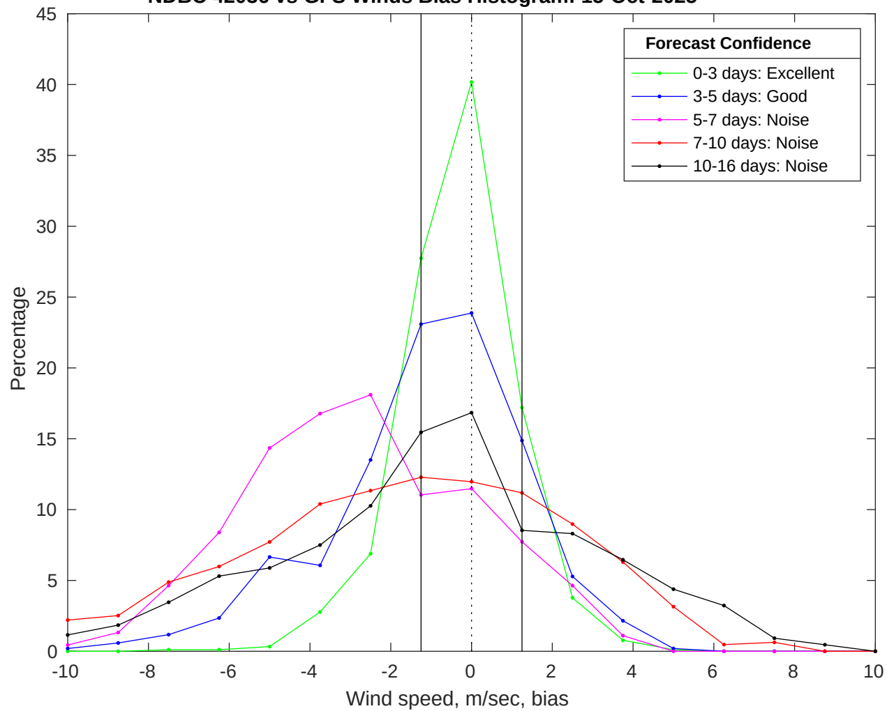
NDBC 42036 vs GFS Winds Bias Histogram: 15-Oct-2025
