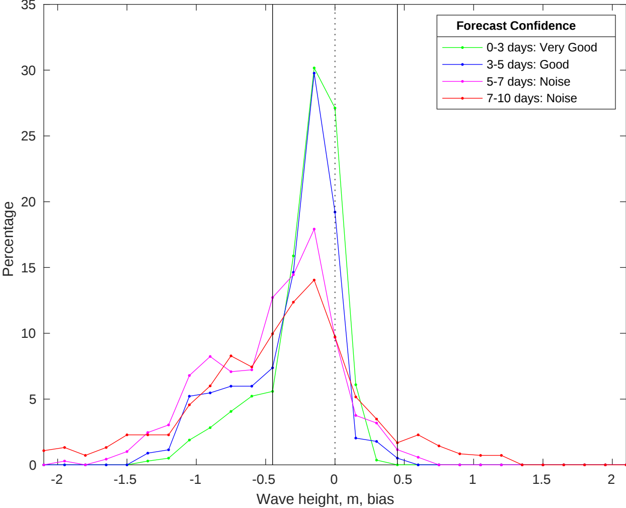
NDBC 42040 vs CMEMS Waves Bias Histogram: 15-Oct-2025
