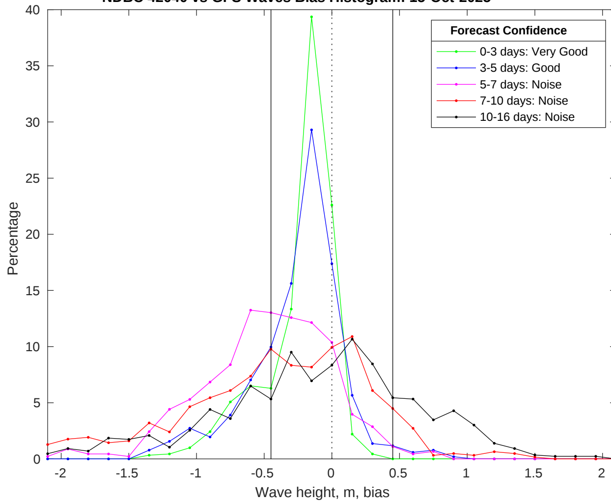
NDBC 42040 vs GFS Waves Bias Histogram: 15-Oct-2025
