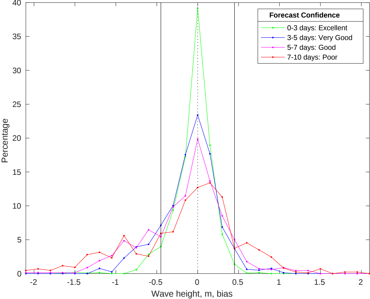
NDBC 44008 vs CMEMS Waves Bias Histogram: 15-Oct-2025
