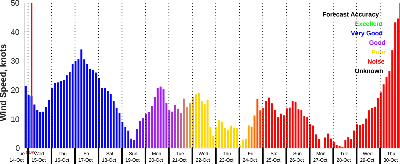
GFS Wind Speed Forecast for NDBC 44008 from 14-Oct-2025 20:00:00 to 30-Oct-2025 20:00:00
