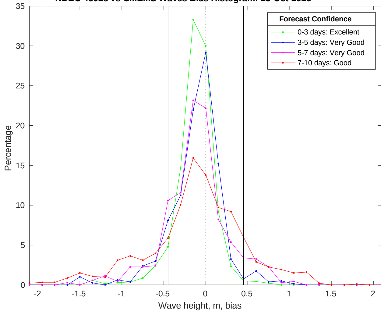
NDBC 46028 vs CMEMS Waves Bias Histogram: 15-Oct-2025
