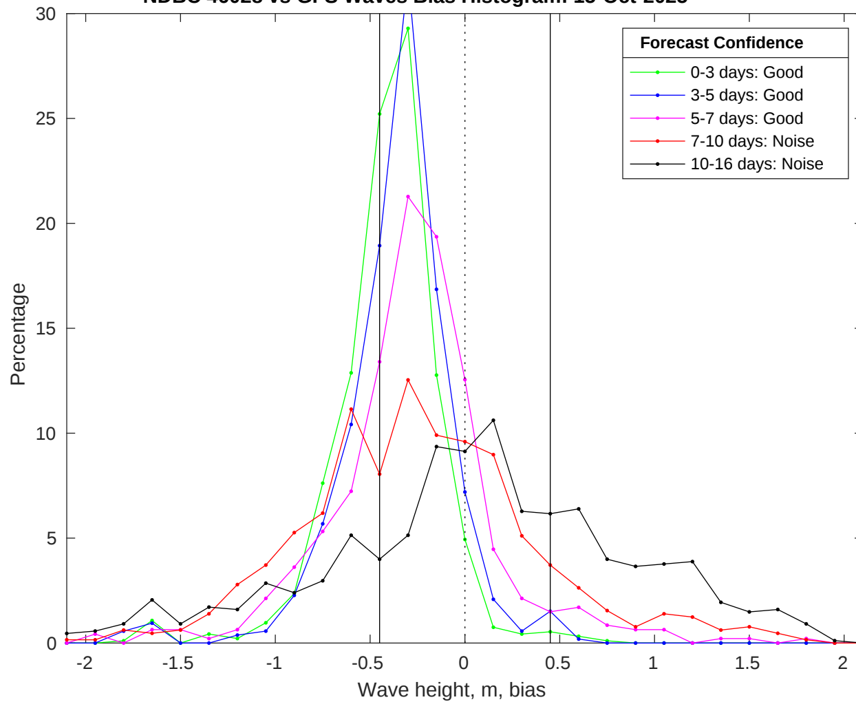
NDBC 46028 vs GFS Waves Bias Histogram: 15-Oct-2025
