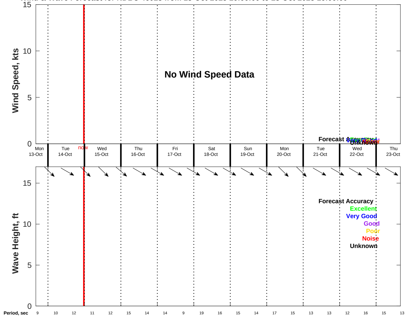
Wind & Wave Forecast for NDBC 46028 from 13-Oct-2025 16:00:00 to 23-Oct-2025 16:00:00
