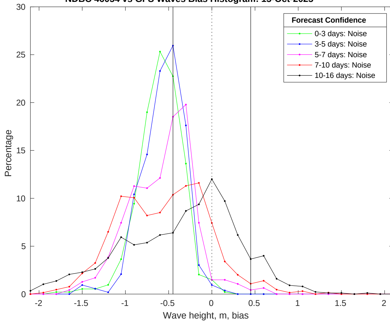
NDBC 46054 vs GFS Waves Bias Histogram: 15-Oct-2025
