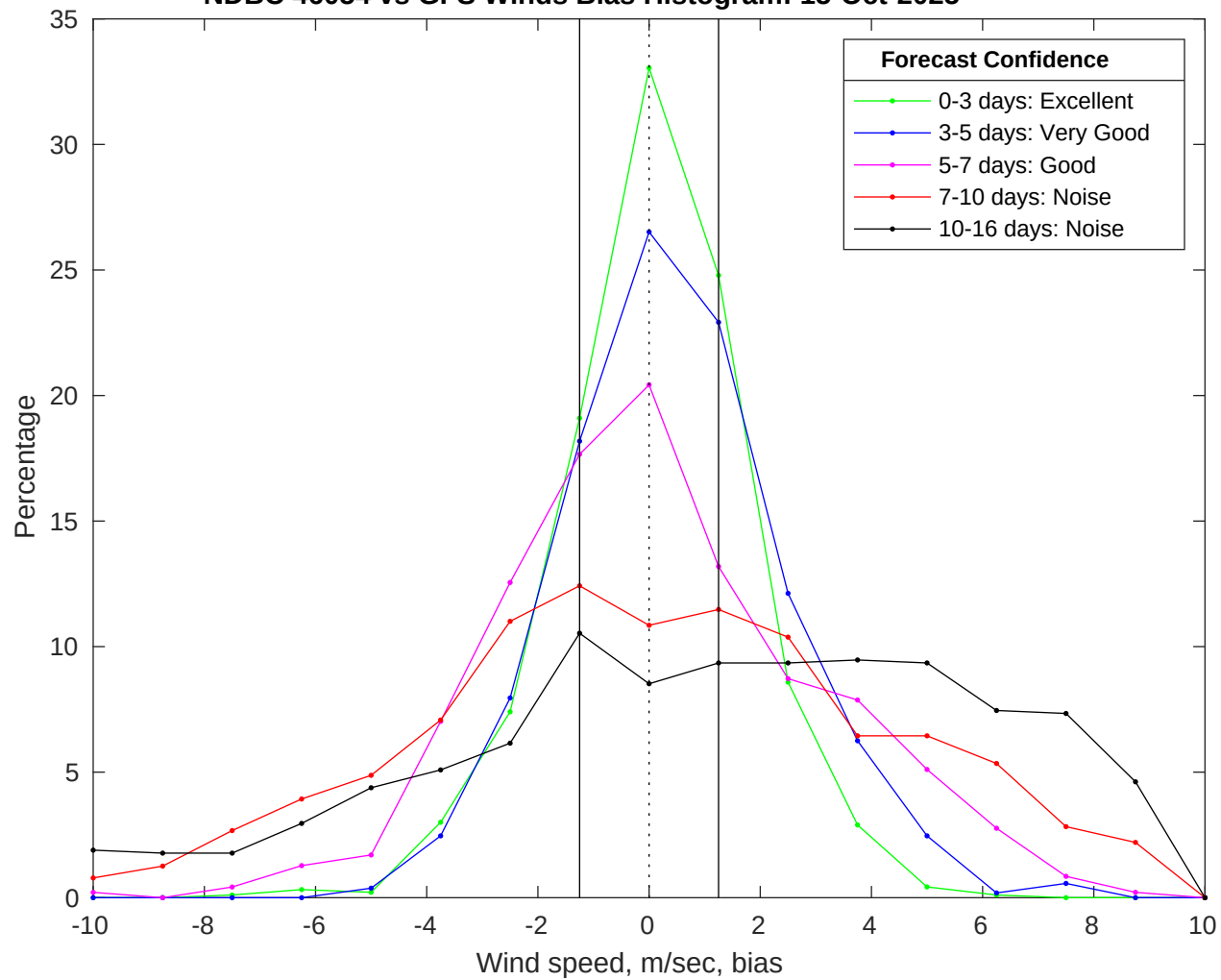
NDBC 46054 vs GFS Winds Bias Histogram: 15-Oct-2025
