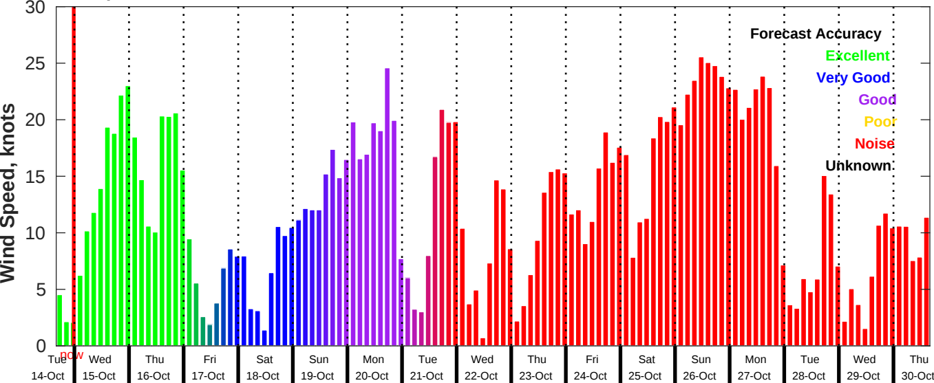
GFS Wind Speed Forecast for NDBC 46054 from 14-Oct-2025 16:00:00 to 30-Oct-2025 16:00:00
