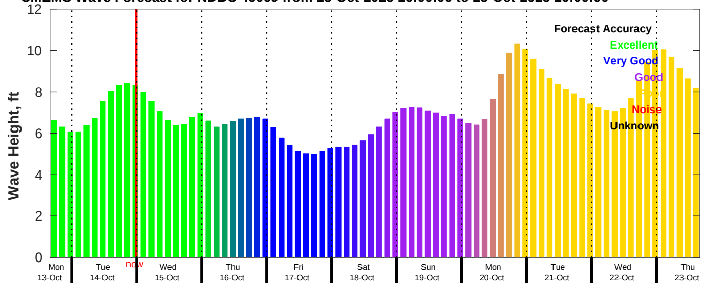
CMEMS Wave Forecast for NDBC 46069 from 13-Oct-2025 16:00:00 to 23-Oct-2025 16:00:00
