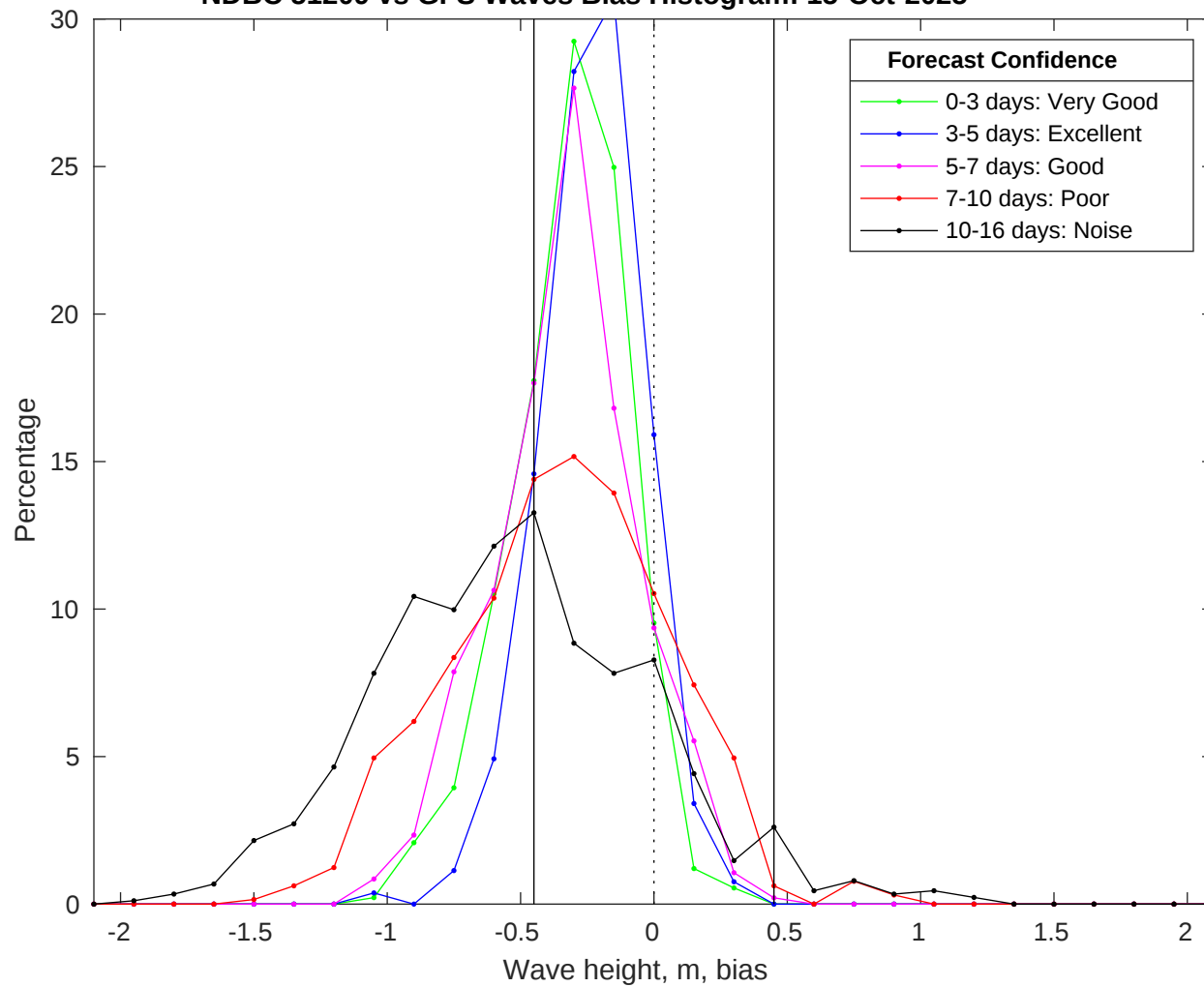
NDBC 51209 vs GFS Waves Bias Histogram: 15-Oct-2025
