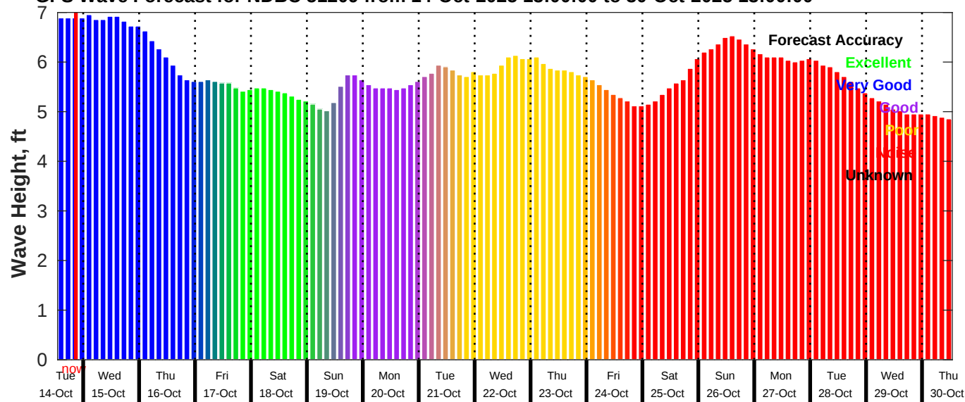
GFS Wave Forecast for NDBC 51209 from 14-Oct-2025 13:00:00 to 30-Oct-2025 13:00:00
