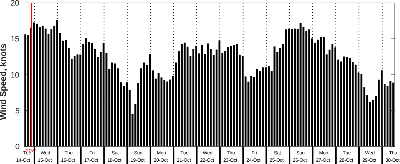
GFS Wind Speed Forecast for NDBC 51209 from 14-Oct-2025 13:00:00 to 30-Oct-2025 13:00:00
