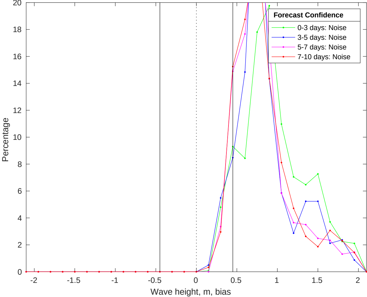
NDBC 51211 vs CMEMS Waves Bias Histogram: 15-Oct-2025
